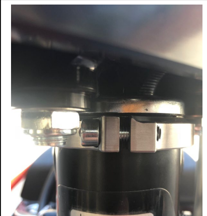
This shows the pinch bolt area with proper clearance to the bolt head at full lock.
