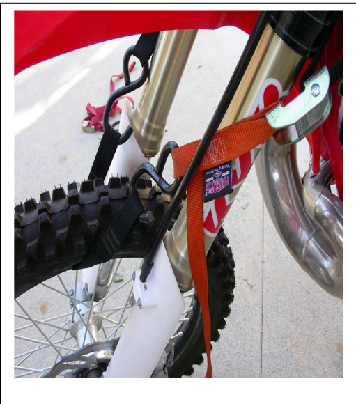
Run a tie down through the front wheel, up and over the back bone to secure the forks in place. This is very important as the forks can roll away from the bike once the triple clamp is off.
