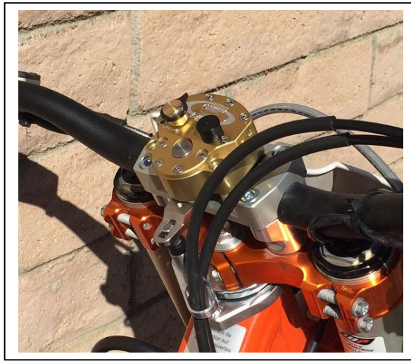
This shows the tower pin centered in the middle of the slot of the link arm. If yours is not centered you may have the lower perches reversed and need to correct the problem or you could damage your stabilizer internally.
