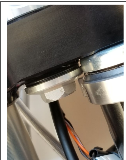
This picture shows the bolt rotated so the flat of the bolt head gives more clearance to the frame bracket.
